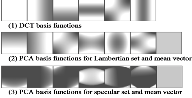
Fig. 4. First six designed lighting patterns
