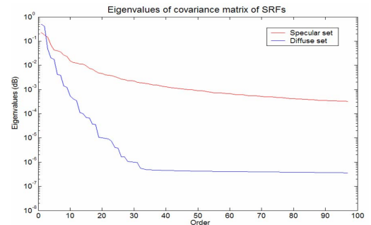
Fig. 3. Eigenvalues of the covariance matrix of SRFs
