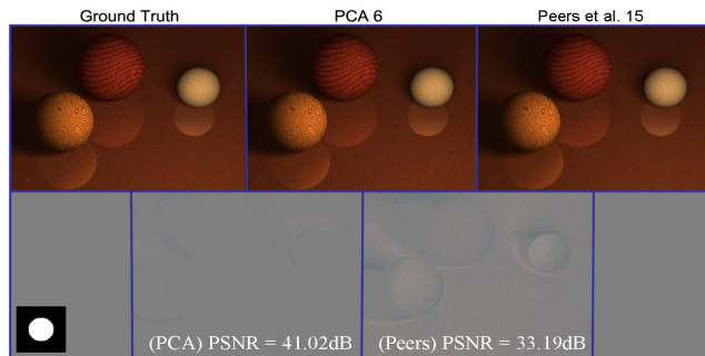
Fig. 6. (1)An object under real lighting(ground truth), (2)A relit image by our proposed method using six images, (3)A relit image by [6] using fifteen images, (4)The difference map between (1) and (2), (5)The difference map between (1) and (3)
