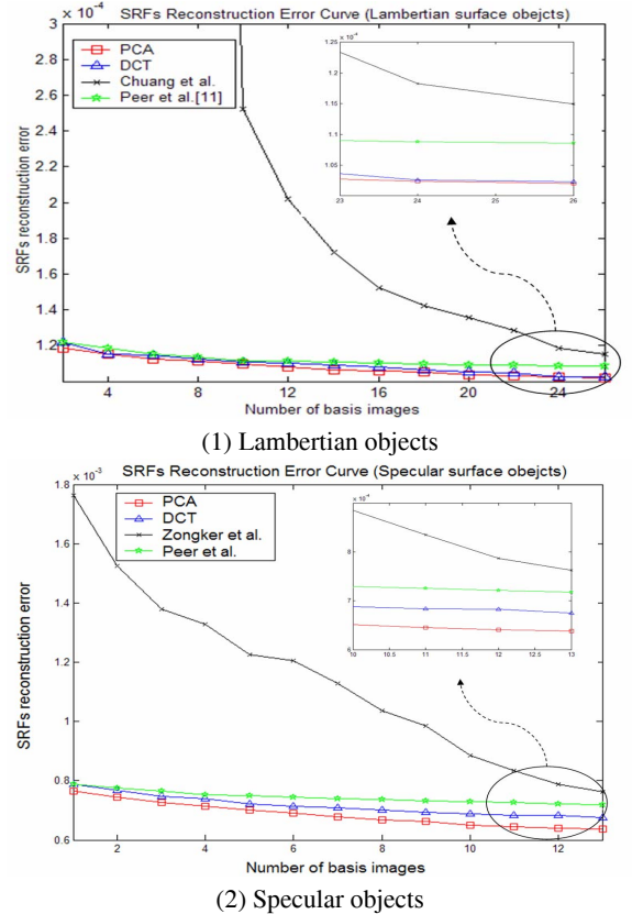
Fig. 5. Comparison with another relighting algorithm
