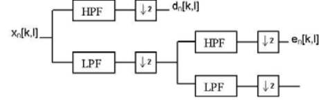
Fig. 1. A two stage filter bank.
