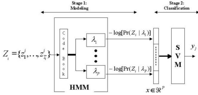
Fig. 1. A block diagram of the proposed framework
