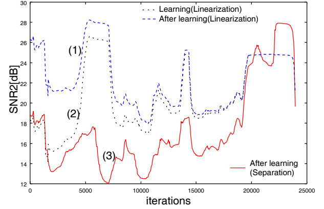
Fig. 3. Learning curve for linearization block.
