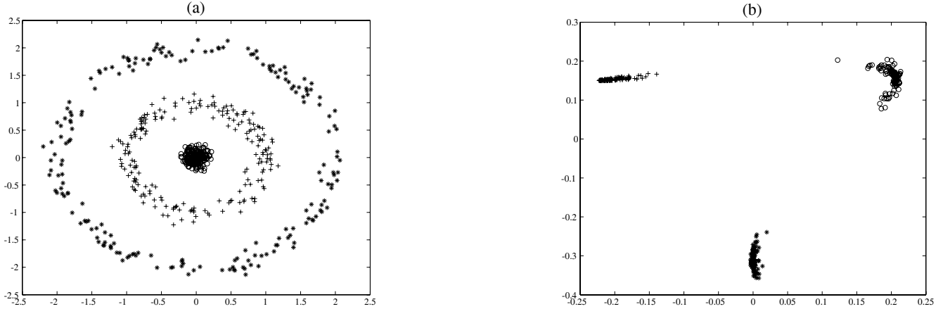
Fig. 2. (a) synthetic data consisting of three classes. The first is represented by \circ , the second by + and the third by \star . (b) Gives the projection of the whole examples on the first two axes using the sequential approach. A gaussian kernel was used with \sigma = 1 .
