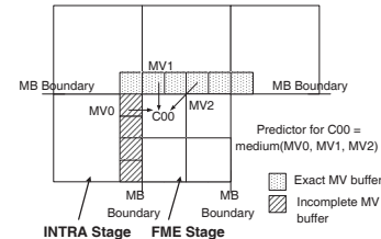
Fig. 4. Incomplete MV predictors used in FME stage.
