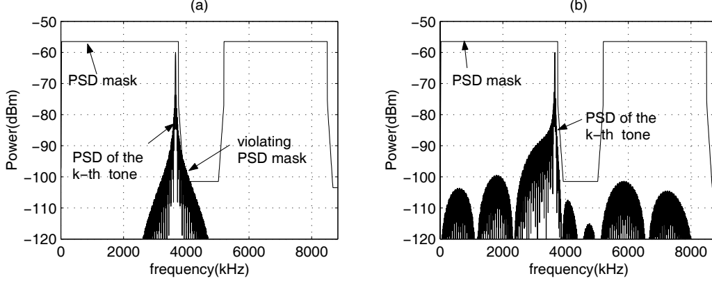
Fig. 3. Comparison of PSD for (a) the frequency shifted window and (b) the per tone window.
