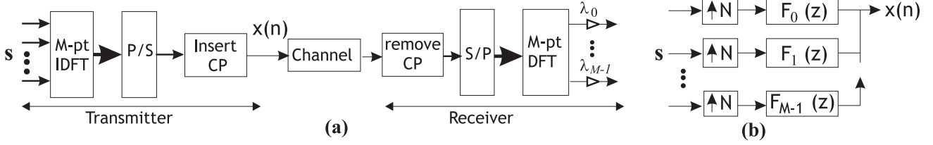
Fig. 1. (a) DMT system (b) Filterbank representation of the transmitter.
