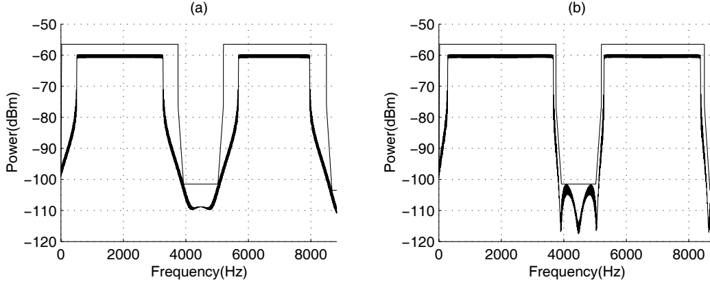
Fig. 4. PSD for transmitted signal x(n) : (a) the frequency shifted window case; (b) the per tone window case.
