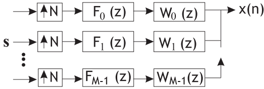
Fig. 2. DMT transmitter with per tone window W_k(z)
