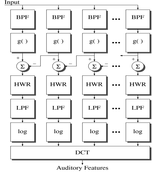
Fig. 2. The bandpass filtered version of the input is non-linearly compressed. The difference operation between lower and higher channels approximates a spatial derivative. The half-wave rectification followed by the smoothing filter picks out the peak. The DCT is performed to decorrelate the signal.
