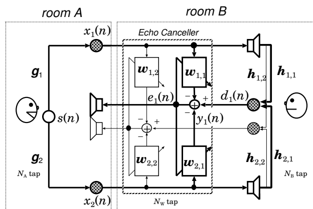
Fig. 1. Teleconferencing using SAEC
