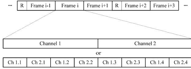
Fig. 3. Bitstream structure (R: random access info)
