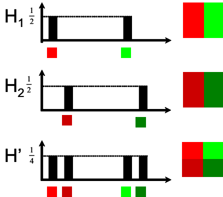
Fig. 1 Using histogram averaging on DCDs
