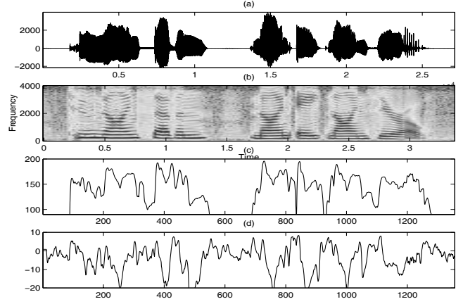
Fig. 1. For the digit sequence '2979890', we show the (a) waveform, (b) spectrogram, (c) entropy of the Mel-filtered spectrum sequence, and (d) entropy of the MFCC sequence.
