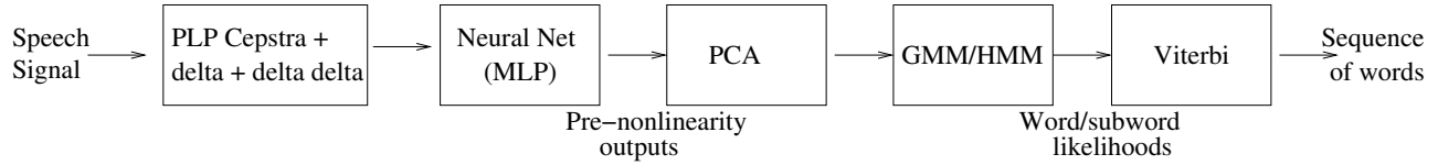
Fig. 1. Block diagram of the tandem feature extraction scheme.
