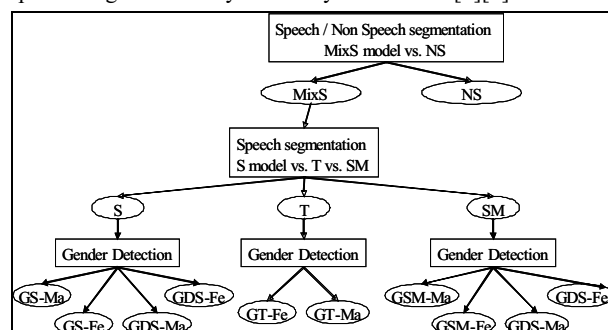
Figure 1: Hierarchical acoustic segmentation
