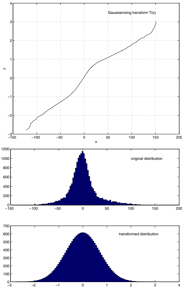
Figure 1: Example of transform and distributions.
