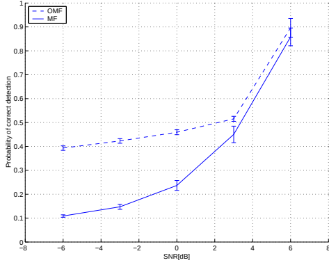
Fig. 1. Mean P_D using the OMF and MF detectors in Beta-distributed noise, as a function of SNR. The vertical lines indicate the standard deviation of the corresponding P_D .
