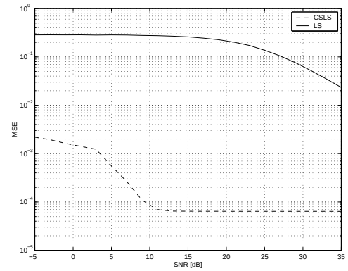
Fig. 4. Mean-squared error in estimating a set of AR parameters using the LS estimator and the CSLS estimator.
