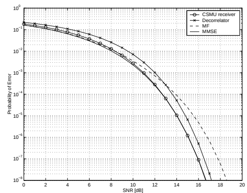
Fig. 2. Probability of bit error with 5 users, \rho = 0.2 , and A_i/A_1 = 0.5 for i = 2, 3, 4, 5 , as a function of SNR.
