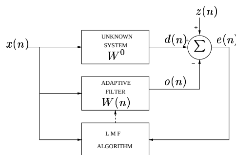
Fig. 1. LMF applied for System Identification.
