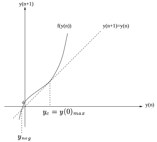
Fig. 3. Equilibrium points: case 2 ( y_c = y(0)_{max} ).
