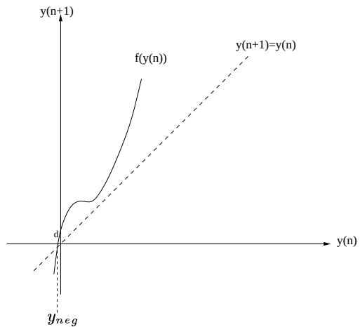
Fig. 4. Equilibrium points: case 3 ( y_c and y(0)_{max} complex).
