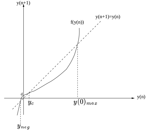
Fig. 2. Equilibrium points: case 1 ( y_c \ll y(0)_{max} ).
