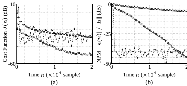
Figure 2: Comparison of convergence among the MCN (—+—), MCFLMS (—Δ—), and NMCFLMS (—o—) algorithms for the random three-channel system, excited by a random BPSK sequence. Trajectories of (a) the cost function J(n) , and (b) the normalized projection misalignment (NPM) \|\epsilon(n)\|/\|\mathbf{h}\| vs. time n are shown for one typical run of the three algorithms.
