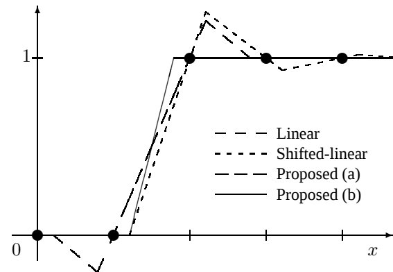
Fig. 3. Interpolation of a unit step function.
