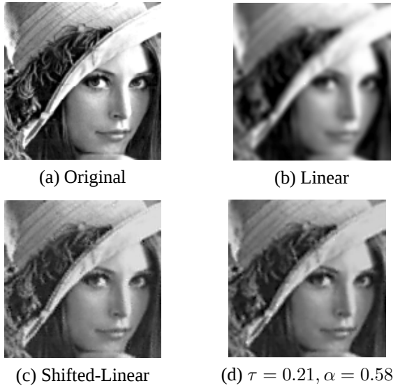
Fig. 4. Rotated Images of “Lena”
