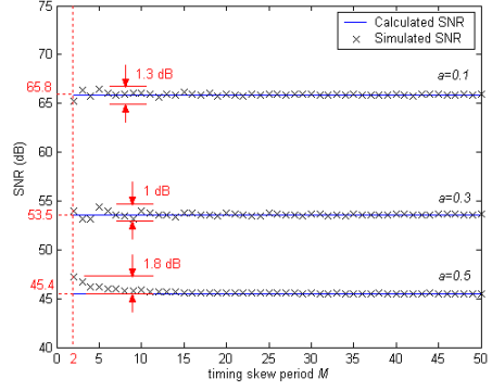
Fig.6 Comparison of simulated & calculated SNR vs. timing-skew period M and normalized frequency a ( \sigma_{rm} = 0.1\% )
