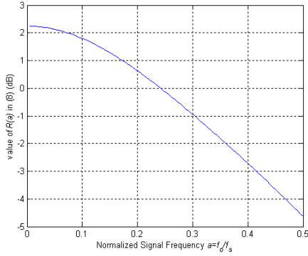
Fig.4 A plot of variation of the R(a) in (9a) vs. normalized frequency a=f_o/f_s
