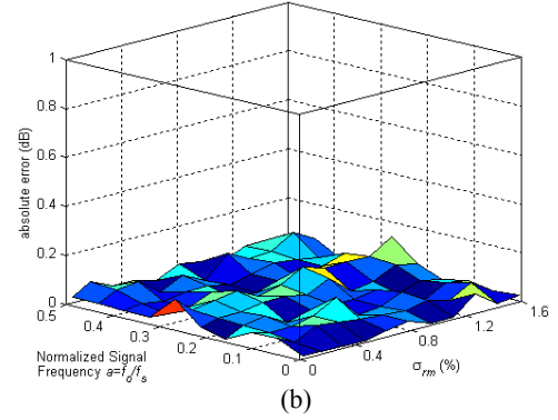
Fig. 5 (a) Simulated SNR & (b) Absolute error between the simulated and calculated SNR of nonuniformly sampled-and-held sinusoid vs. normalized frequency a and standard deviation \sigma_{rm} (with 1000 times Monte-Carlo Simulations and M=50 )
