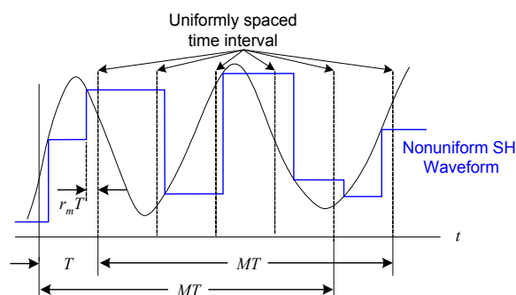
Fig.1 Nonuniformly Sampled-and-Held Signal
