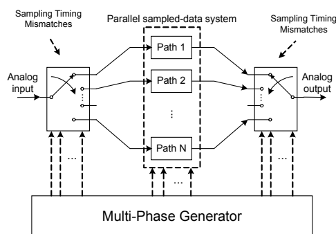
Fig.2 General parallel sampled-data systems structure
