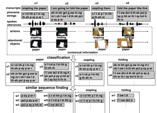
Fig. 2. Word-like unit segmentation. Spoken utterances are categorized into several bins that correspond to temporally co-occurring actions and attentional objects. Then we compare any pair of spoken utterances in each bin to find the similar subsequences that are treated as word-like units.
