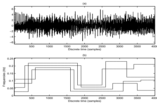
Fig. 1. (a): Test signal; (b): Normalized frequencies of the sinusoids.
