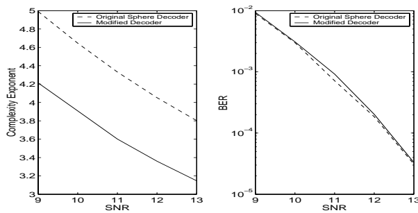
Fig. 2. Complexity Exponent and BER for N=20 with QPSK
