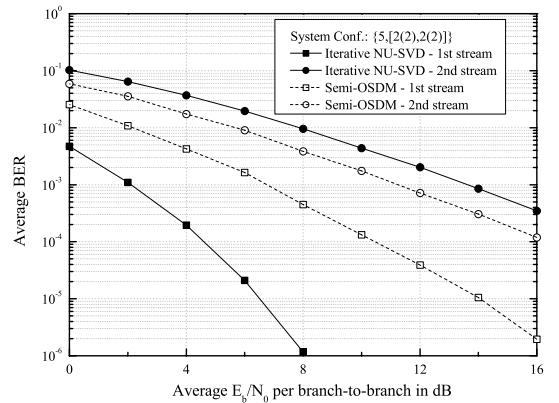
Fig. 3. Average BER results versus average E_b/N_0 per branch-to-branch for systems with N_m = 2 \forall m .
