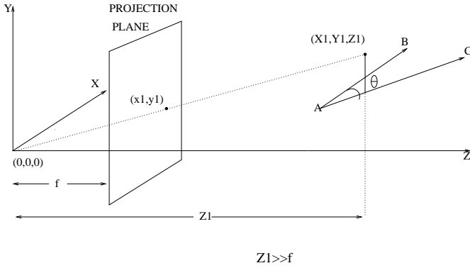
Fig. 1. Imaging Geometry
