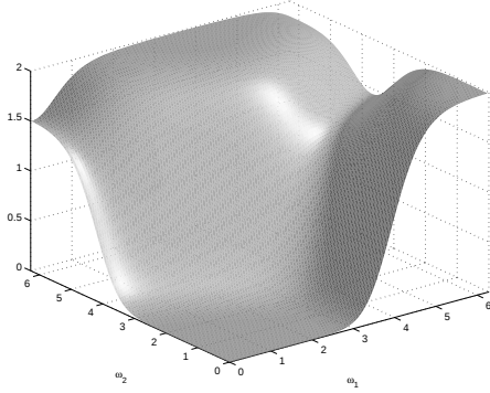
Fig. 2. The error kernel E(\omega) corresponding to the fourth-order interpolation prefilter.
