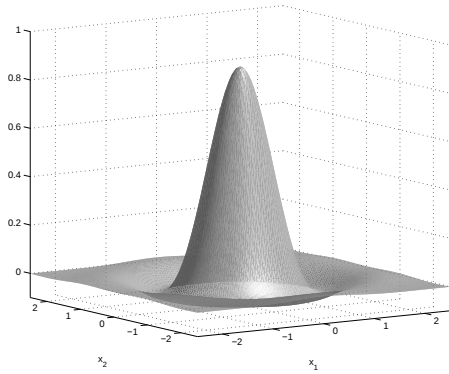
Fig. 4. Impulse response of the combined prefilter and reconstruction function for fourth order: (\eta_4 \otimes \tilde{h}_2)(\mathbf{x}) .
