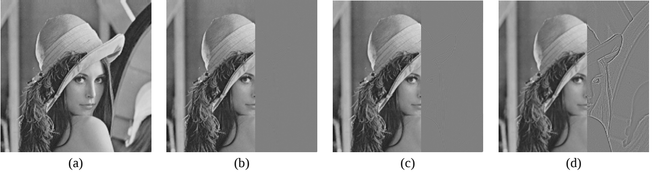
Fig. 3. The results of the test image “lena” for the fourth-order hex-spline using different prefilters. (a) Prefiltering in the Fourier domain with the interpolation prefilter 1/\hat{h}^3 . (b) Prefiltering in the spatial domain with the recursive filter \tilde{h}_2 . (c) Prefiltering in the spatial domain with \tilde{h}_3 . (d) Without prefilter.
