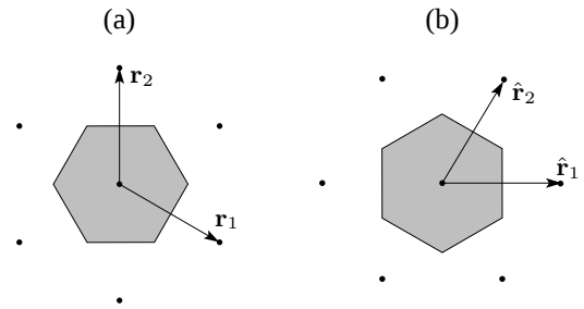
Fig. 1. (a) The regular hexagonal lattice of the second type and its Voronoi cell. (b) The dual lattice.
