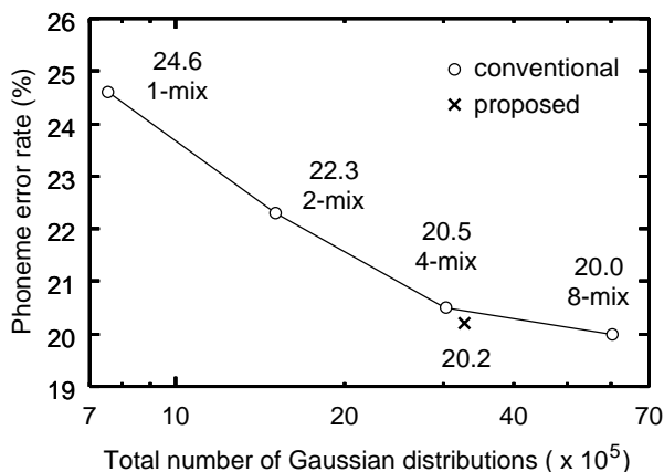
Fig. 3. Recognition results by the conventional method and the proposed method (male).
