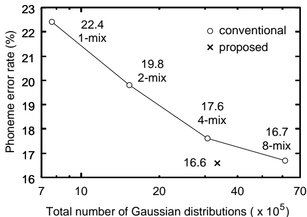
Fig. 4. Recognition results by the conventional method and the proposed method (female).
