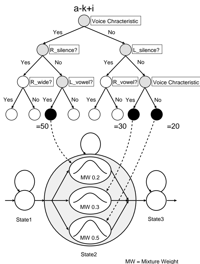
Fig. 2. Integration of voice characteristic dependent acoustic models.
