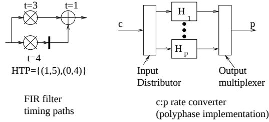
Figure 4: Multirate FIR filter structure.
