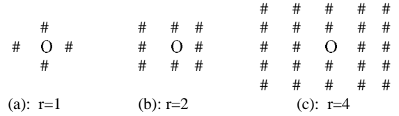
Figure 2: Neighborhood configuration
