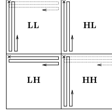
Figure 4: Scanning of the different subband images
