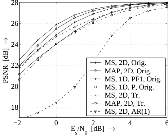
Figure 6: Performance of the image transmission system for the "Goldhill" image ( R = 0.36 bpp, L = 3 )
