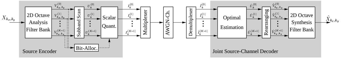
Figure 5: Experimental image transmission system
