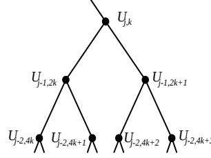
Figure 2: (a) Binary tree of Haar scaling coefficients. (b) MWM construction: At scale j , we form the wavelet coefficient as the product W_{j,k} = A_{j,k} U_{j,k} . Then, at scale j - 1 , we form the scaling coefficients U_{j-1,2k} and U_{j-1,2k+1} as sums and differences of U_{j,k} and W_{j,k} (normalized by 1/\sqrt{2} ).
