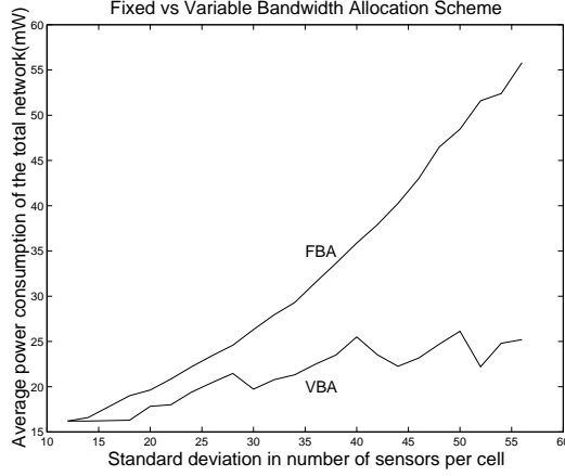
Fig. 5. Power consumption for different frequency allocation schemes
