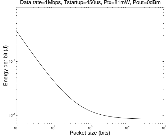
Fig. 1. Effect of startup transient
