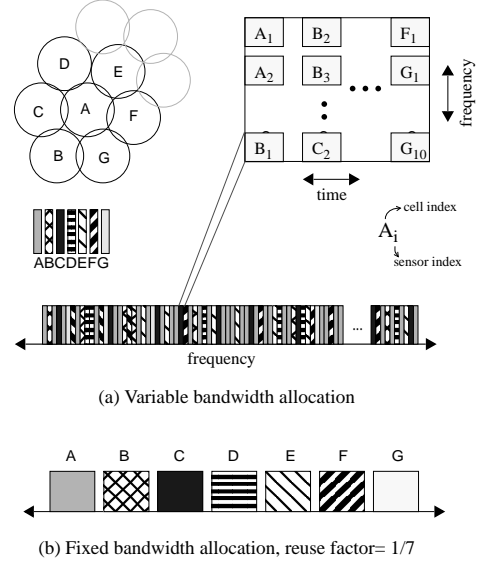
Fig. 4. Bandwidth allocation schemes
