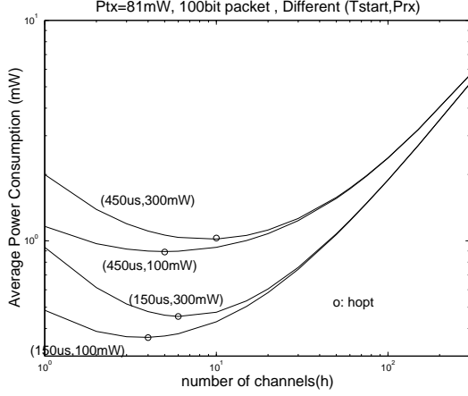
Fig. 3. Energy with different (T_{startup}, P_{rx})
