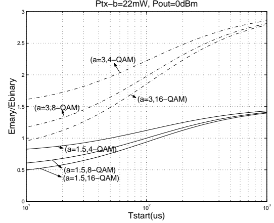
Fig. 6. Energy Saving vs Overhead( \alpha )
