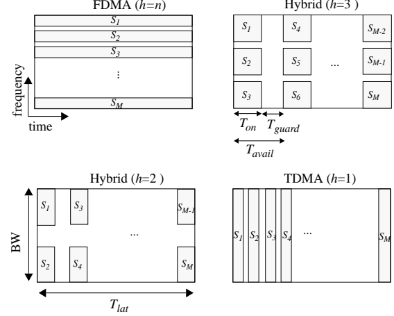
Fig. 2. Multiple access methods
