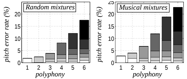
Fig. 4. Pitch error rates for multipitch estimation in different polyphonies. Bars represent the overall error rates, and the different shades of gray the error cumulation in iteration.
