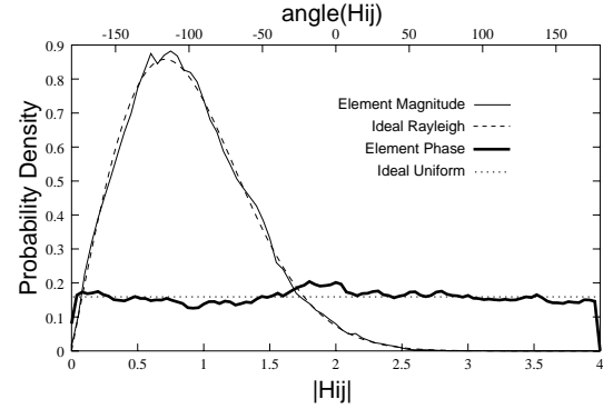
Fig. 5. Empirical PDFs for the magnitude and phase of the 10 \times 10 \mathbf{H} matrix elements.
