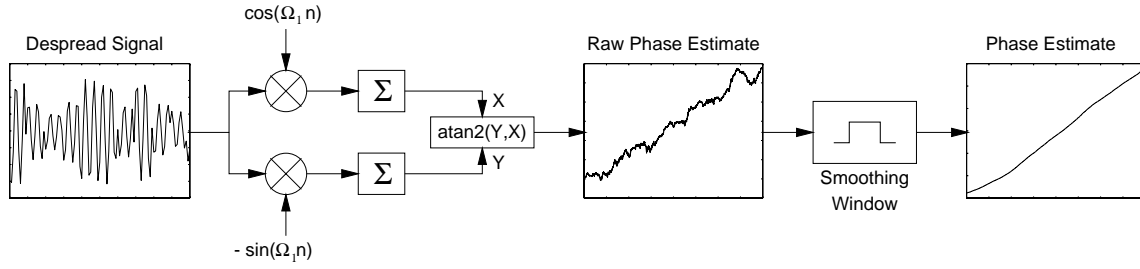
Fig. 3. Carrier phase recovery method
