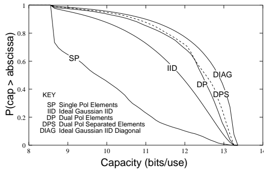
Fig. 8. CCDFs for 2x2 channels employing different types of polarization/spatial separation.
