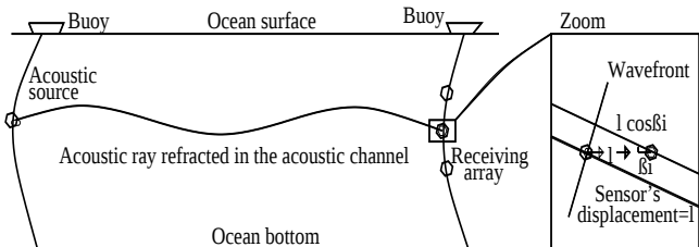
Fig. 1. Ray propagation and sensor displacement offset.
