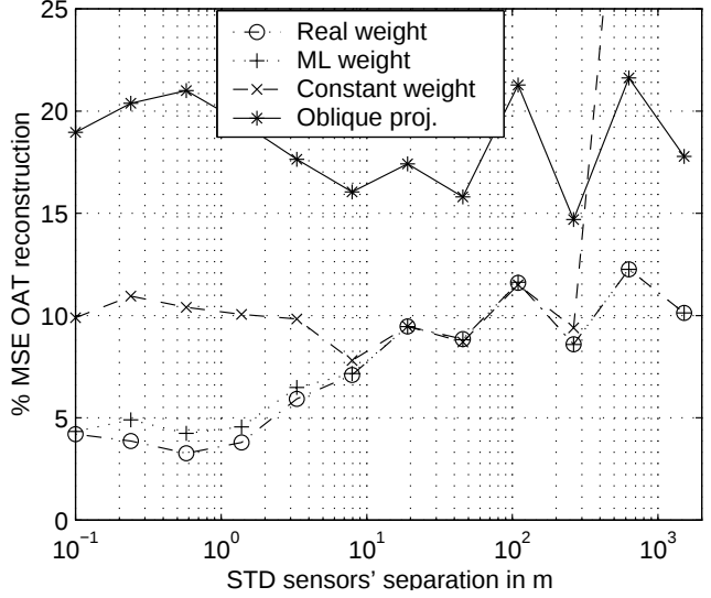
Fig. 2. MSE of OAT reconstruction by four inversions
