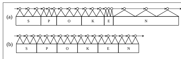
Fig. 1. Illustration of the word “spoken” before (a), and after (b) duration normalization. Corresponding HMM states are shown above each phone segment and are mapped to the approximate phone region they model.
