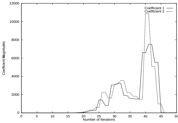
Fig. 2. Trajectory of w_{1,k} and w_{2,k} for \mu = 0.33 for a 2-adaptive filter in a cyclo-stationary signal environment described in Section 5
