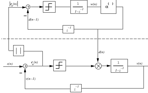
Fig. 2. Adaptive Delta Modulator.
