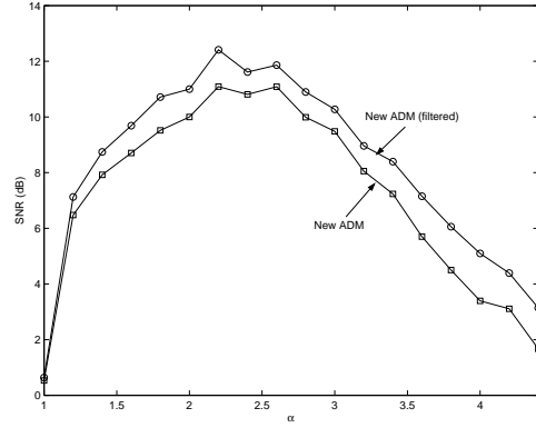
Fig. 7. SNR performance of the new ADM versus the exponent term \alpha .
