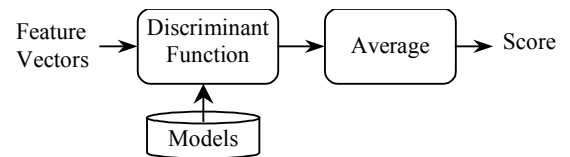
Figure 4: Classifier structure.
