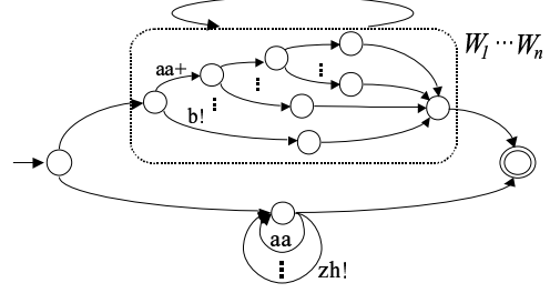
Fig. 4. The topology of FST M for the phoneme network model with fillers.
