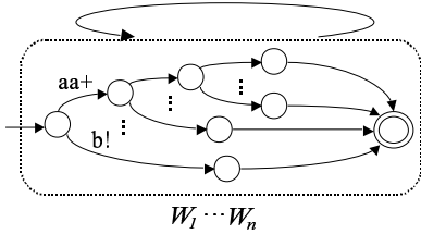
Fig. 3. The topology of FST M for the lexicon-based phoneme network model.
