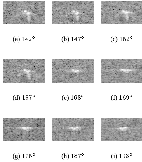
Fig. 6. SLICY canonical target images ( 54 \times 54 ) at elevation 39^\circ and different azimuth angles. Image in (e) is inserted in Fig. 5.
