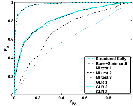
(b) Case 2 (SNR = 10dB)
