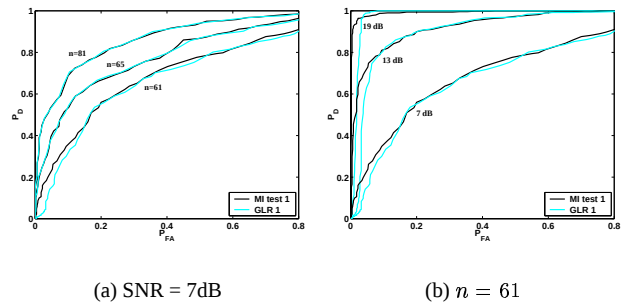
Fig. 2. Comparison of GLR and MI tests for Case 1 by (a) increasing n with fixed SNR and (b) increasing SNR with fixed n ( m_A = 60, m_B = 40 ).
