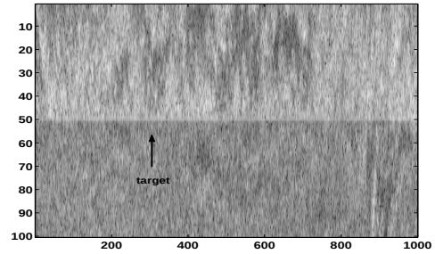
Fig. 7. Image realigned along the extracted boundary. SLICY target is located at column 305 with |a| = 0.015 . This target is just above the minimal detectable threshold for the three tests investigated in Fig. 8.
