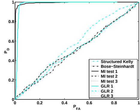
(a) Case 1 (SNR = 19dB)
