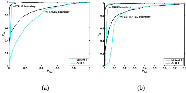
Fig. 4. Comparison of ROC curves for Case 1 using true boundaries and (a) biased boundaries moved downward by one pixel; (b) estimated boundaries in each snapshot (True values: m_A = 60, m_B = 40, n = 61 ).
