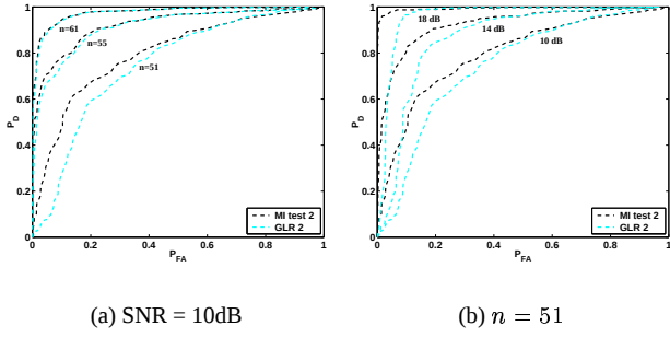
Fig. 3. Comparison of GLR and MI tests for Case 2 by (a) increasing n with fixed SNR and (b) increasing SNR with fixed n ( m_A = 50, m_B = 50 ).
