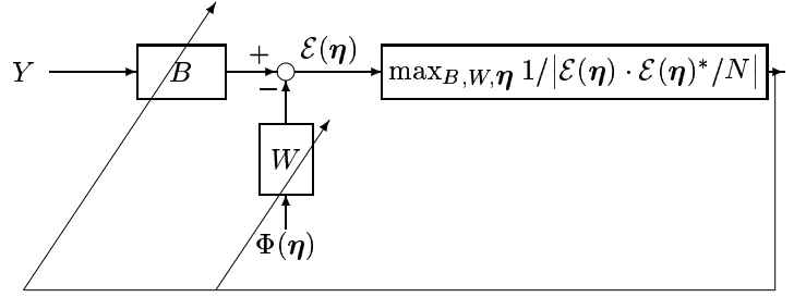
Fig. 1. Proposed MIMO adaptive equalization scheme.
