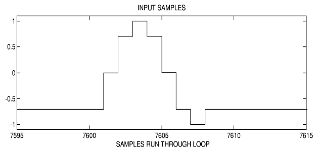
Figure 3. Analog levels represented by a burst of digital input samples entering the probe.
