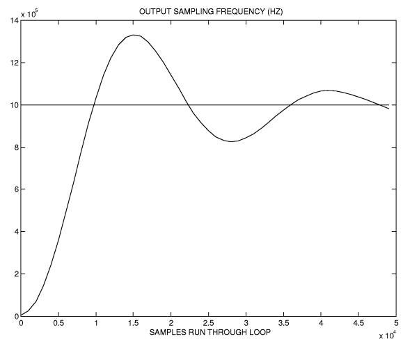
Figure 6. Long-term plot of the output sample rate of the simulated control loop.
