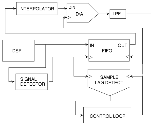
Figure 1. Block Diagram of the probe, showing the reconstruction circuit.
