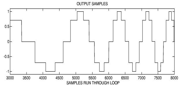
Figure 4. Analog output samples after repeated bursts of digital input samples.
