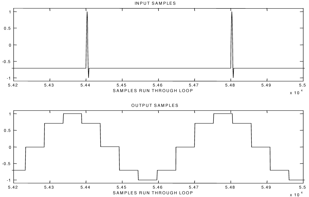
Figure 5. Input and output samples of the sample buffering system plotted on the same time base.
