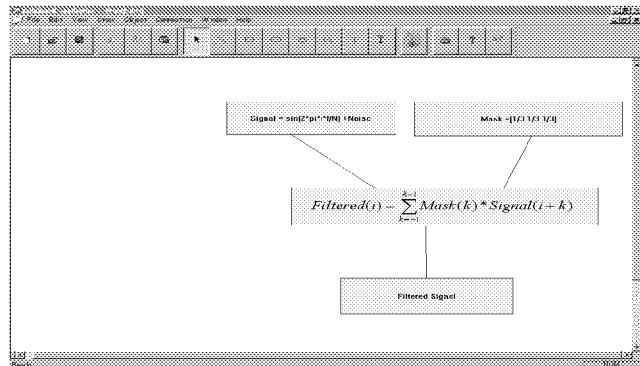
Figure 4 : Convolution Operation.
