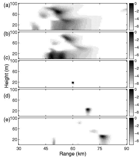
Figure 6: Range-height ambiguity surfaces for uncertainty in the layer thickness value. The source was at 60 km range and 18.6 m height; the true layer thickness was 110 m. Layer thickness values are: (a) 70 m (b) 90 m (c) 110 m (d) 130 m (e) 150 m.
