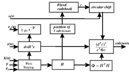
Fig. 3 Codebook Search in AVQ-CELP
