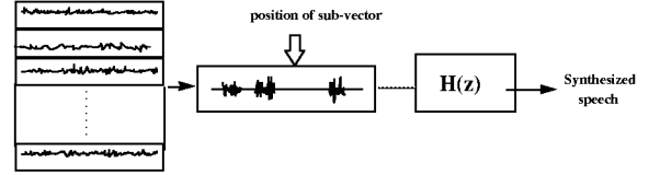
Fig.1 The Algebraic VQ CELP
