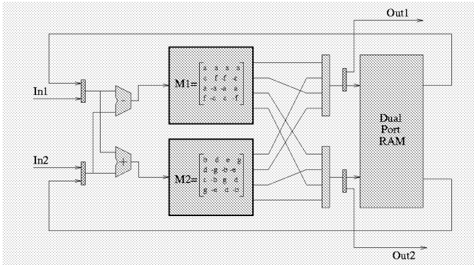
Figure 4: DCT Architecture
