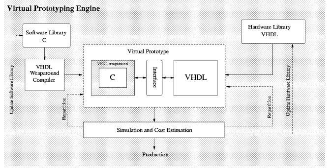
Figure 2: Virtual Prototyping Engine (VPE)
