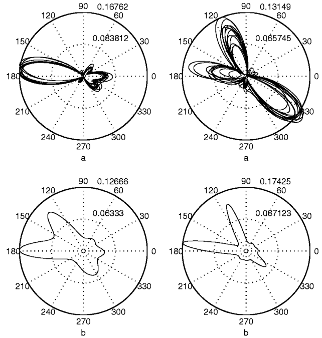
Figure 3. LOSWLS Scenario: DOA Estimates Via (a) Beamforming (b) Subspace Smoothing Approach
