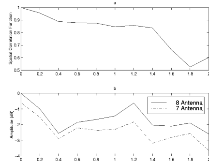
Figure 2. NOLOS Moving MT Scenario: (a) Spatial Correlation Between the Current SS and 1st SS, (b) Diversity Comparison
