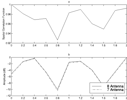
Figure 1. LOSWLS Moving MT Scenario: (a) Spatial Correlation Between the Current SS and 1st SS, (b) Diversity Comparison
