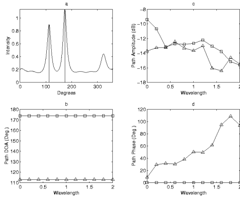
Figure 7. NOLOS Scenario: (a) MUSIC Spectrum, (b) DOA Estimates, (c) Path Amplitudes, (d) Relative Multipath Phases
