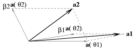
Figure 8. Illustration of SS Change in NOLOS Scenario
