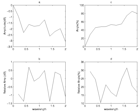
Figure 10. Spatial Signature Variation in NOLOS Scenario: Amplitude Change of the Current SS in Relative to the (a) 1st SS (b) Last SS, Angle Change of the Current SS in Relative to the (c) 1st SS (d) Last SS
