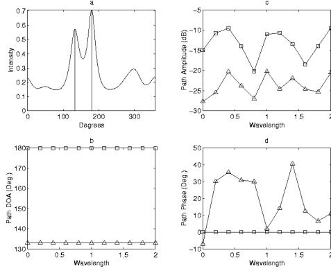
Figure 5. LOSWLS Scenario: (a) MUSIC Spectrum, (b) DOA Estimates, (c) Path Amplitudes, (d) Relative Multipath Phases
