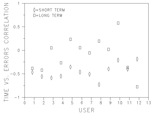
Figure 7: Correlation coefficient between errors and usage time. Squares plot the correlation over all the usage period, diamonds plot the correlation within the performed sessions.
