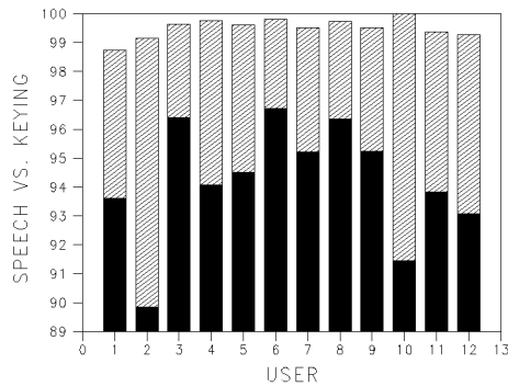
Figure 2: Percentage of operations performed by speech versus keyboard/mouse, by each user. Black bars account for all kinds of actions (i.e. button clicks, field selections, and field assignments). Gray bars only consider field assignments.
