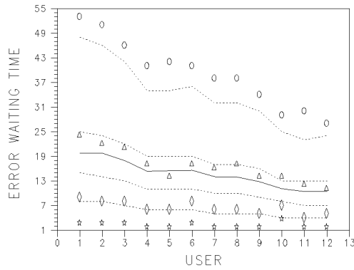
Figure 4: Distribution of the time distances between errors. The sharp line represents the empirical mean. Dotted lines show, from the bottom upward, the .3, .5, .7, and .9 quantiles of the geometric distribution. Symbols represent the same quantiles of the empirical distribution.
