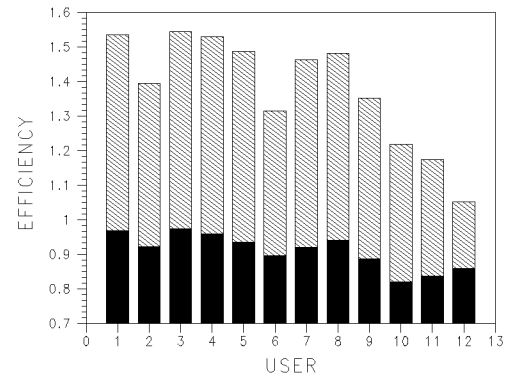
Figure 6: Efficiency measures expressed as the ratio between task size and number of performed actions. The black bar accounts for all single operations, even in case of multiple operation utterances. The gray bar counts multiple operation utterances as single operations.
