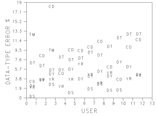
Figure 5: Error rate on different data-types by each user. Data-types are grouped into six categories: CD code, DS description, DT date, DY day, TM time, and YR year.
