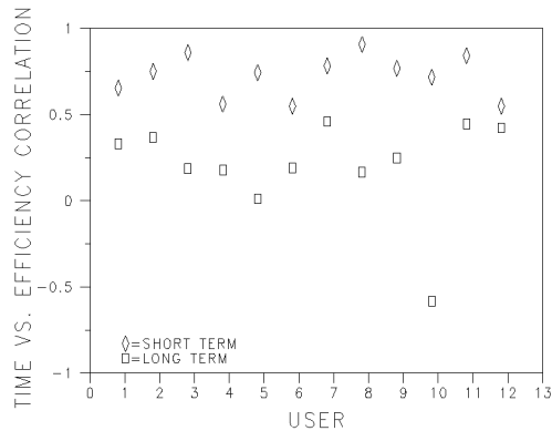
Figure 8: Correlation coefficient between efficiency and time. Squares show the correlation computed overall the usage period, diamonds show the within-session correlation.
