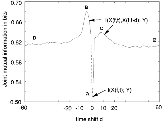
Figure 5: The JMI of the 5-th frequency band as a function of time shift (in frames). Information is gained by using a feature located at a different time (e.g. B, C, D, or E) in addition to the feature from the current frame (located at point A). See the text for a discussion.
