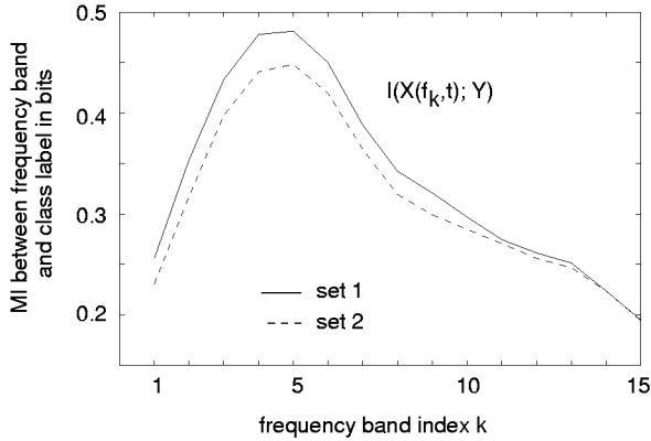
Figure 2: Mutual information as a function of frequency and the classification target variable for two disjunct sets of 100 speakers each. The two speaker sets exhibit similar MI patterns across frequency.
