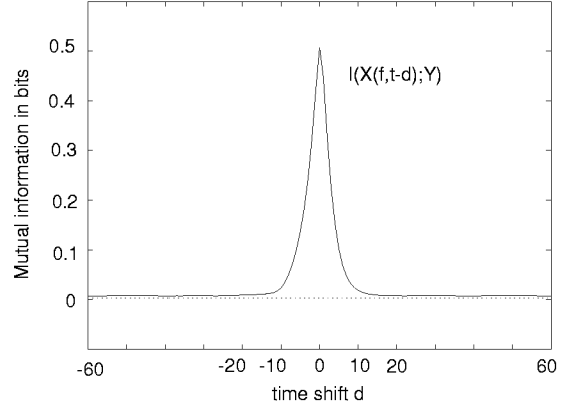
Figure 3: Mutual information as a function of time shift (in frames) and the classification target variable for the 5-th frequency band. The dotted line shows the lower bound (0.0028 bits) which is the mutual information between the 5-th frequency band and scrambled phonetics labels.
