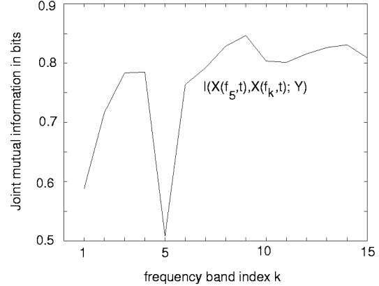
Figure 4: JMI as a function of frequency for a feature point in the 5-th band and a feature point in the k-th band.
