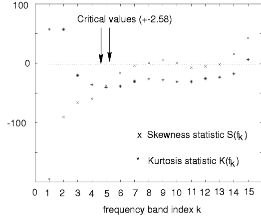
Figure 1: The statistics S and K in each frequency band of the spectrum of 50 speakers.
